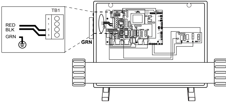
Figure D Terminal Block 240V Wire Connection
